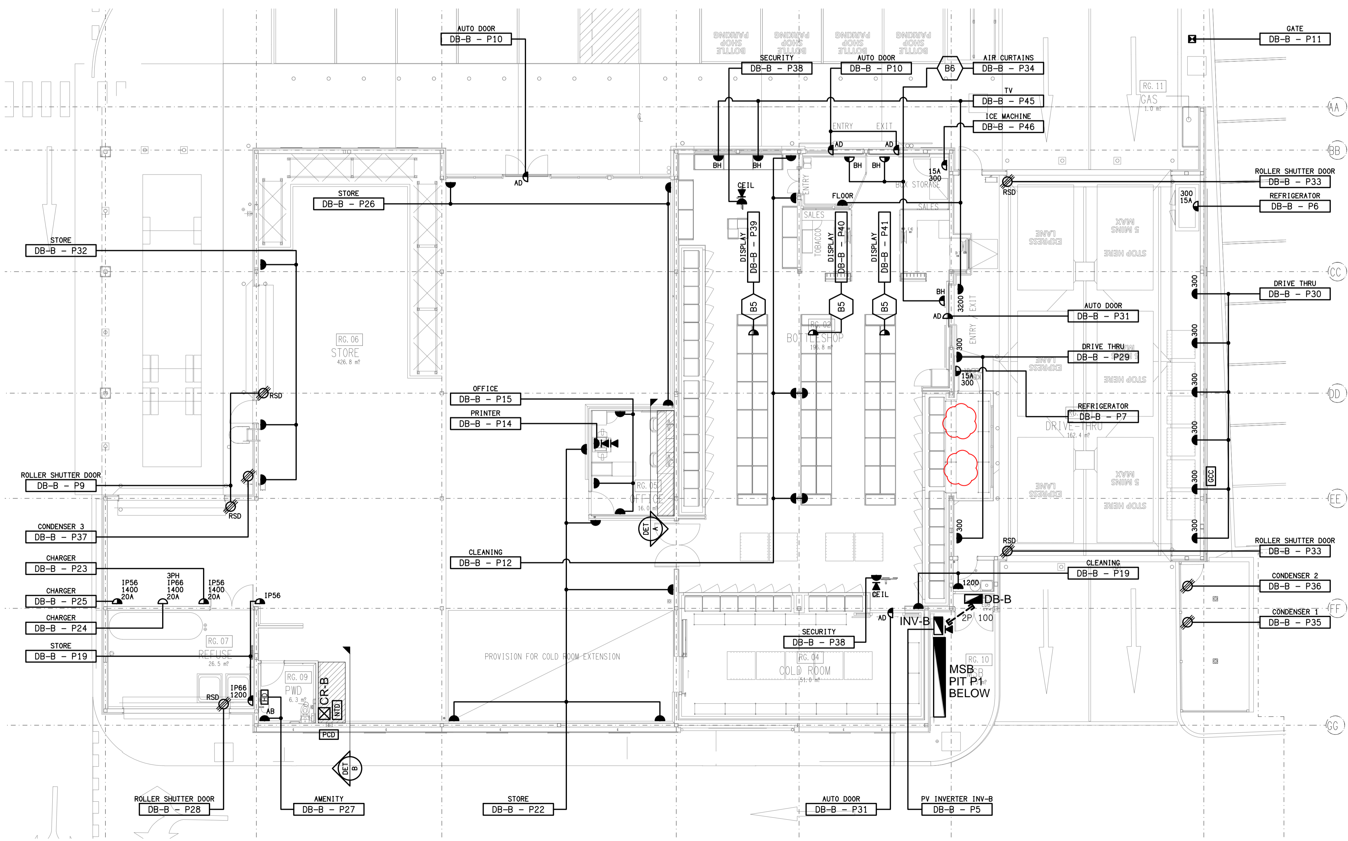
DETAIL D POINT OF SALE & ENTRY FLOOR PLAN SCALE 1: 50
