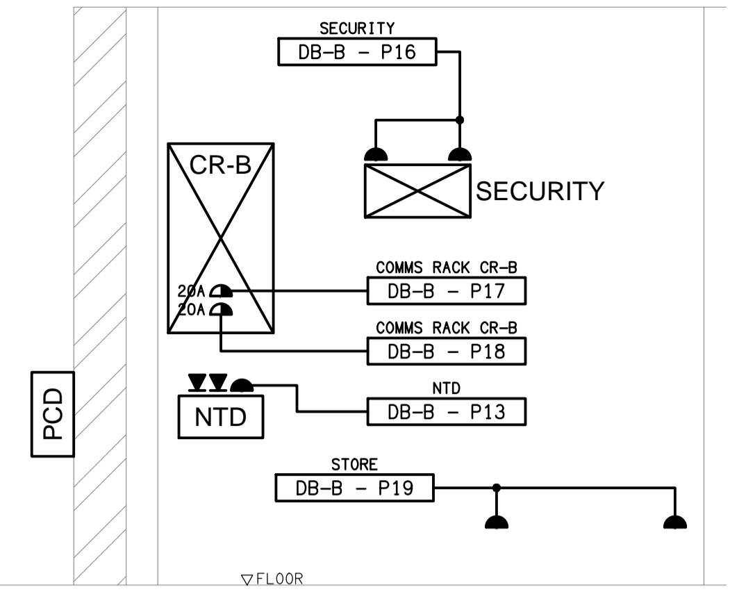
DETAIL B COMMUNICATIONS WALL ELEVATION SCALE 1: 25
